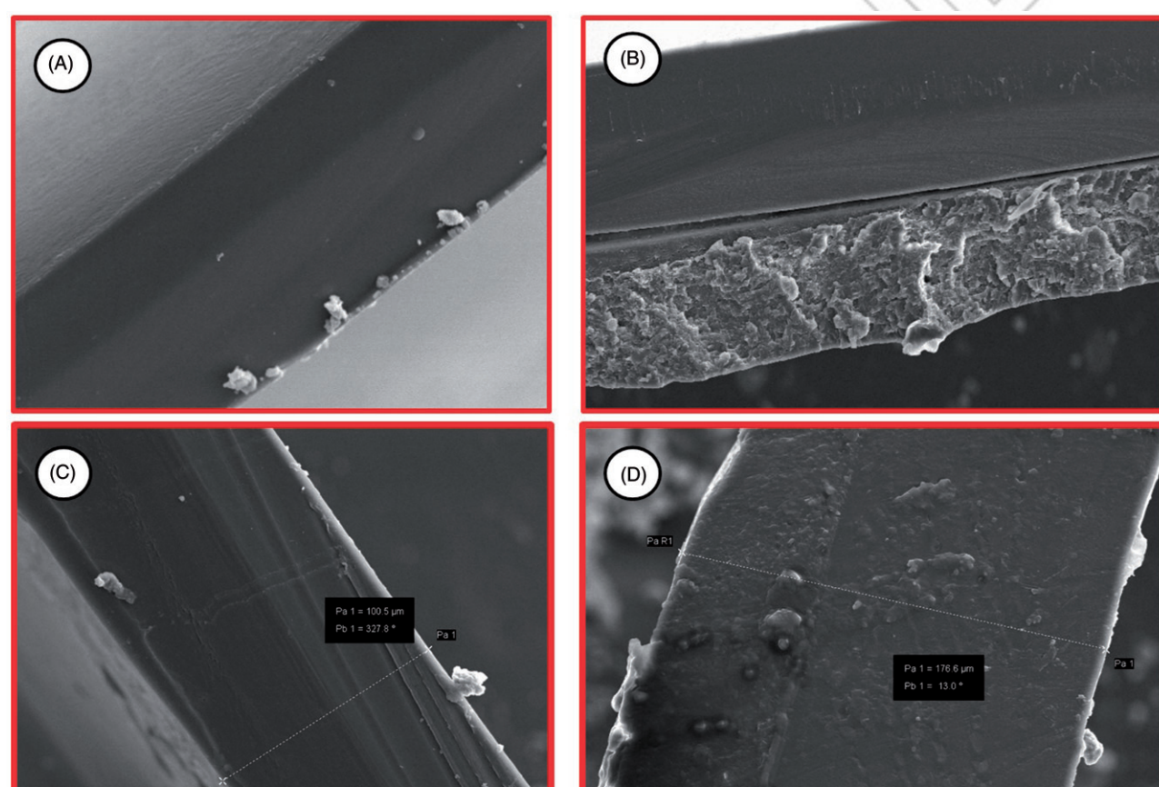
Figure 6. SEM image of the cross-section of a cleaved surface through (A) a non-coated capsule, (B) coated capsule with Eudragit FS and (C) the thickness of cross-section of uncoated capsule, and (D) coated capsule with Eudragit FS.
